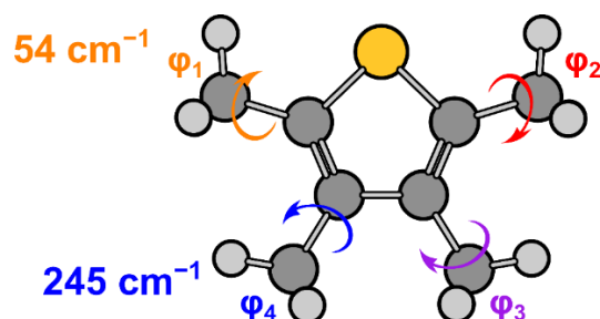
Figure 7. The four-top molecule 2,3,4,5-tetramethylthiophene. The two upper tops \phi_1 and \phi_2 as well as the two bottom tops \phi_3 and \phi_4 are equivalent [190]. The preliminary torsional barriers are given.
