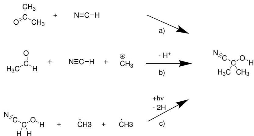
Scheme 1: Possible reactions to form acetone cyanohydrin.
