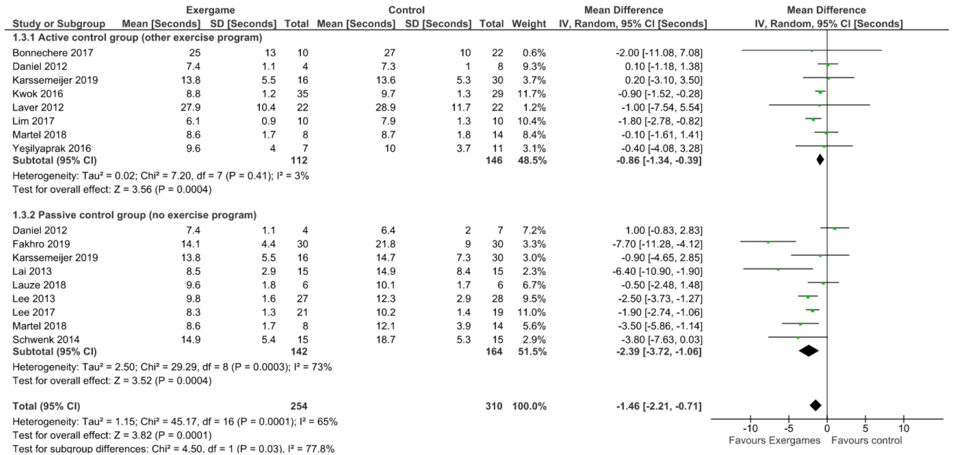
Figure 3: Forest plot for the Timed up and go. Notes: A reduction in the score of the Timed Up and Go means a reduction in fall risk, thus a negative mean difference means a reduction in fall risks in the exergame group.
