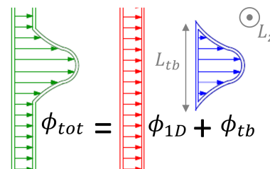
Figure 3: Scheme of additional heat flux \phi_{tb}
