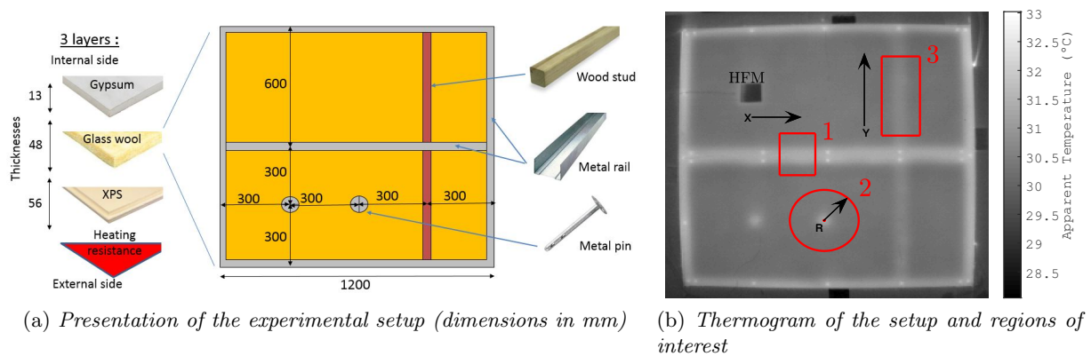
Figure 1: Overview of the setup and thermogram obtained in steady state (25W heating power). Thermal bridges as well as a surface heat flux meter are visible.
