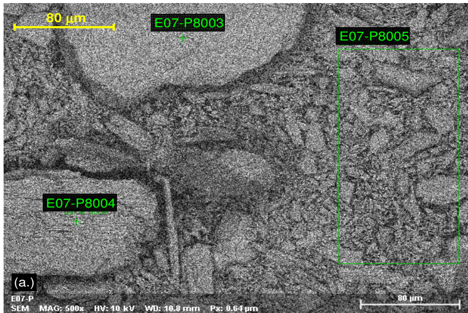
4 5 6 Fig. 3 SEM micrograph of used plaster
