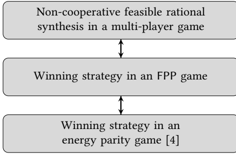
Figure 3: Chain of reductions used in solving the non-cooperative feasible rational synthesis problem.
