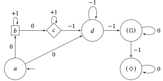
Figure 4: A three-player game. Player 1 has a vacuous qualitative objective and thus only cares about not depleting the resource.
