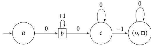
Figure 2: A two-player game with a solution.
