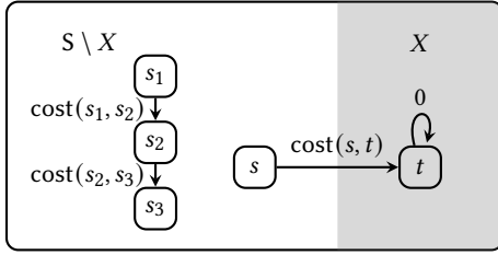
Figure 5: Illustration of the game \hat{\mathcal{G}} arena construction. X is as in Lemma 4.
