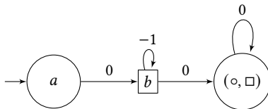
Figure 1: A two-player game without a solution.
